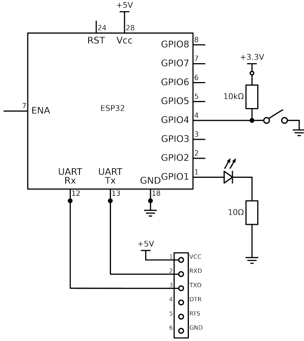
Fig. 2. Example Schematic generated with Schemdraw [10].
